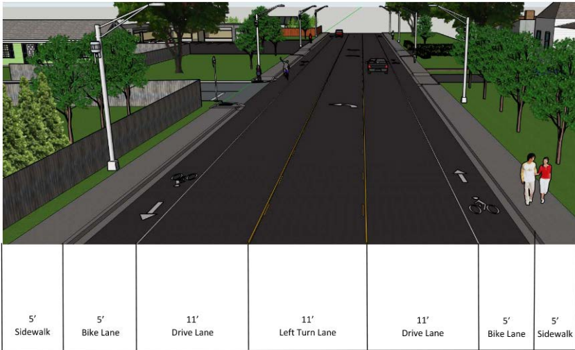
Figure 3 - TYPICAL ROADWAY SECTION
