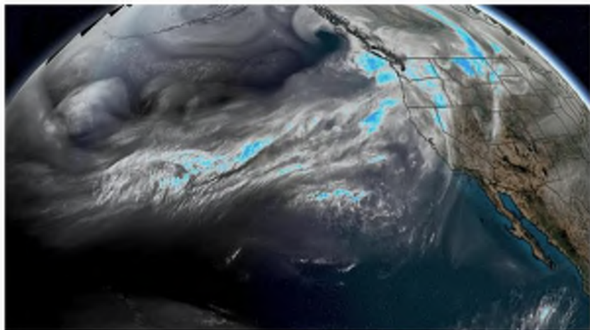
Atmospheric River, January 2021.
