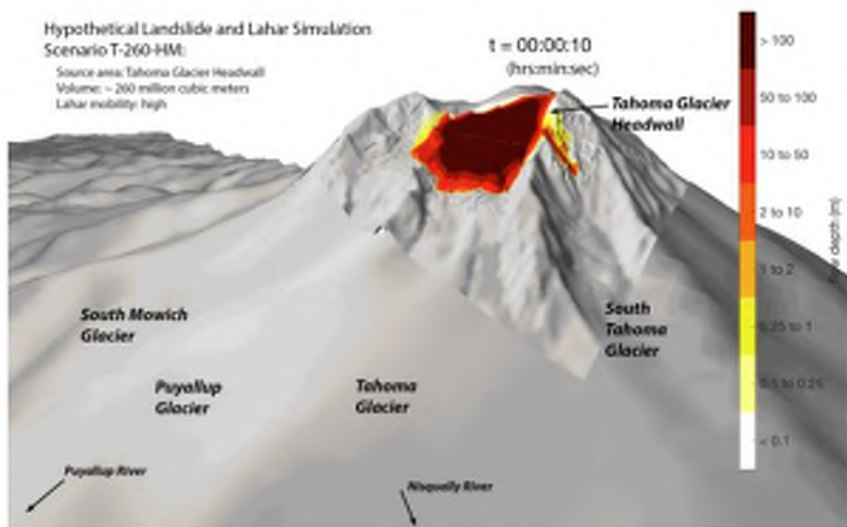
Lahar affecting Nisqually and Puyallup Rivers
