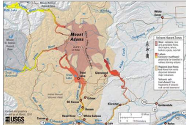
Mount Adams Lahar and Lava Hazard Areas
