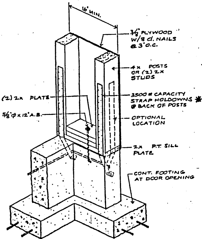
④ STRAP HOLDDOWNS OPTIONAL LOCATION
