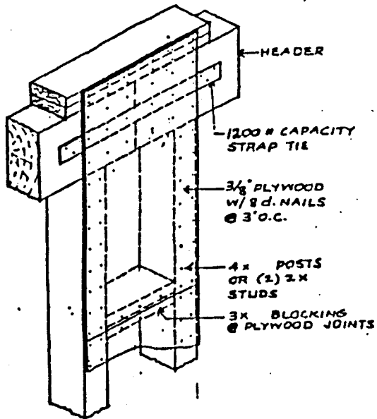
③ HEADER SPLICE
